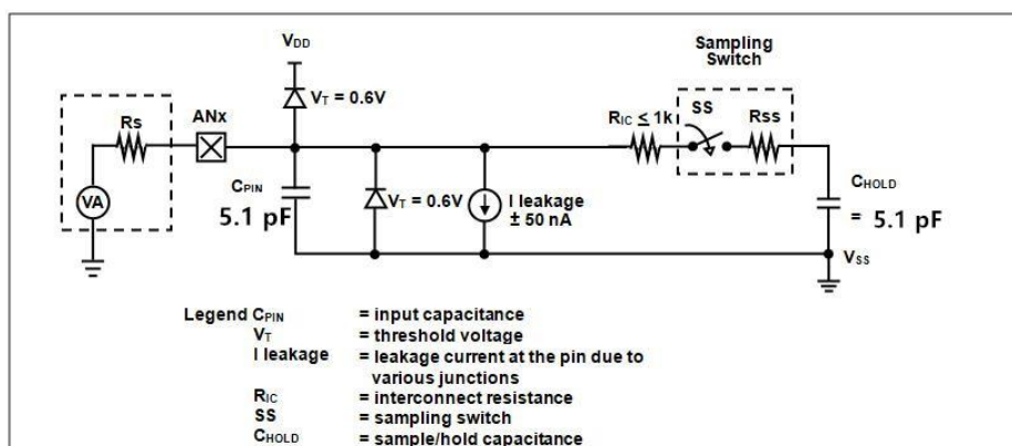
Fig.21: Analog Input Model
