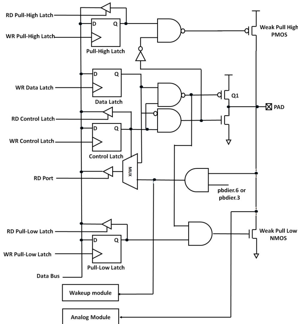
Fig. 18: Hardware diagram of IO buffer with Weak Pull High PMOS & Weak Pull Low NMOS
