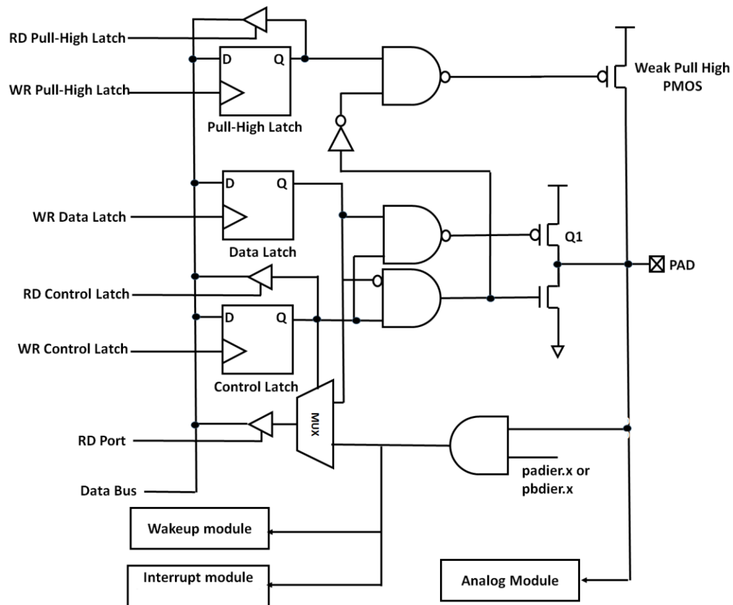
Fig. 17: Hardware diagram of IO buffer with Weak Pull High PMOS
